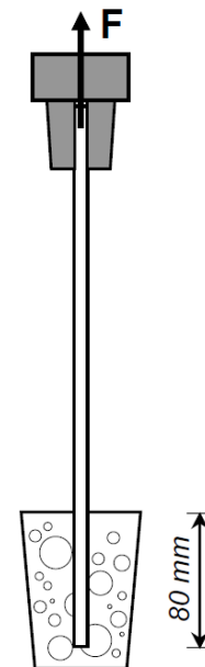
Figure 2. Schematic of the pullout test
